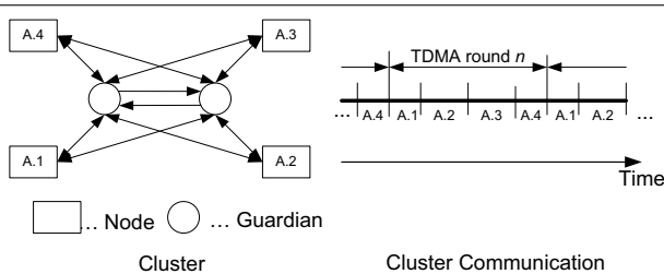
Figure 1. TTA cluster and TDMA schedule
